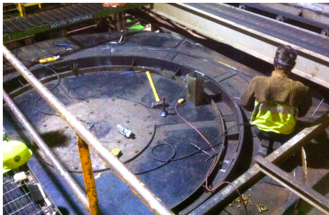
Rebuild Turntable Column Hardboard Collins Products- Klamath Falls, OR
